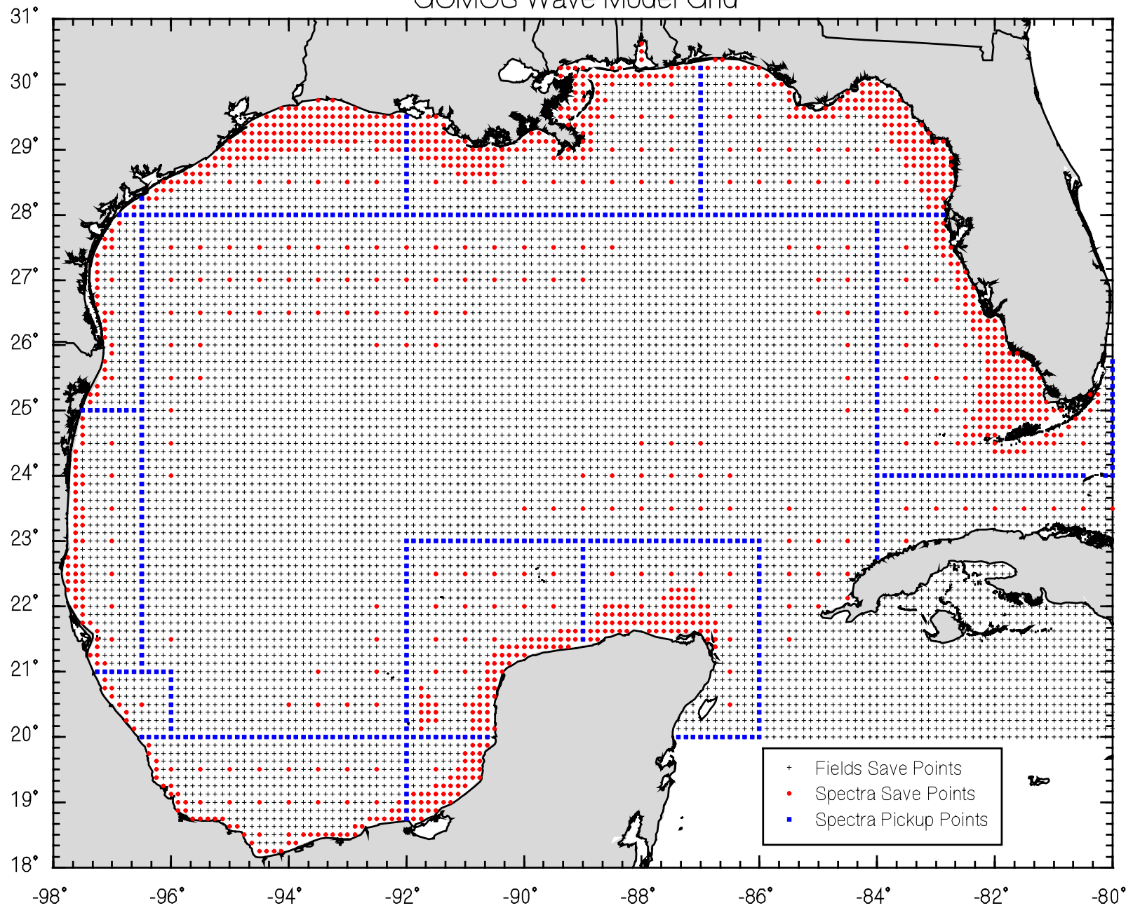
GOMOS Wave Model Grid
